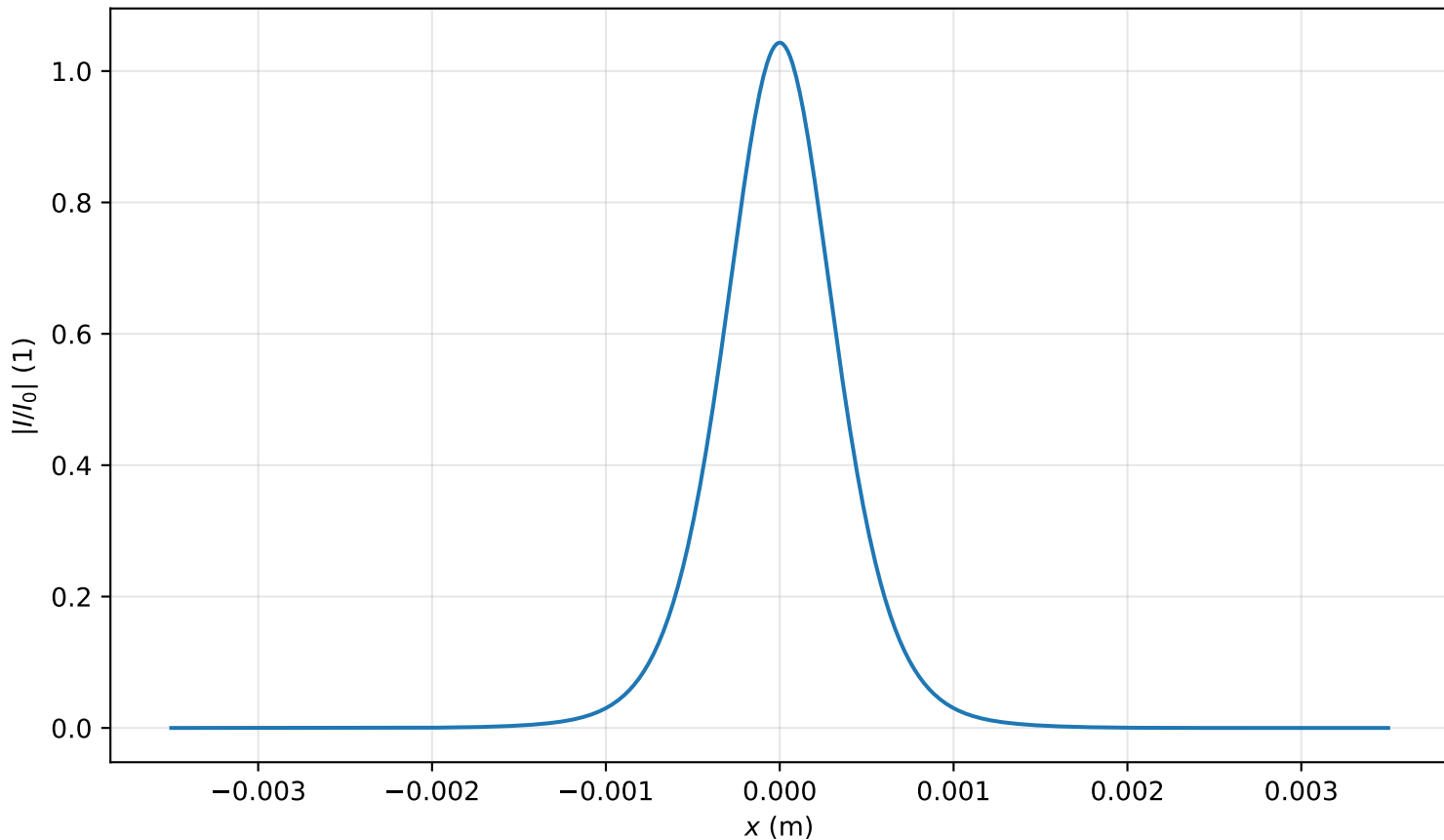
Intensity profile I(x, y = 0, z = 2.229m)/I_0 , P_{in}=0.7P_{cr} , artificial time
